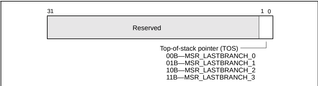
Figure 14-4. MSR_LASTBRANCH_TOS MSR Layout
