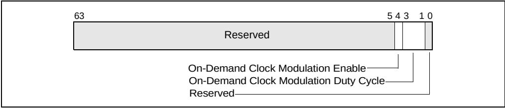
Figure 12-9. IA32_THERM_CONTROL MSR
