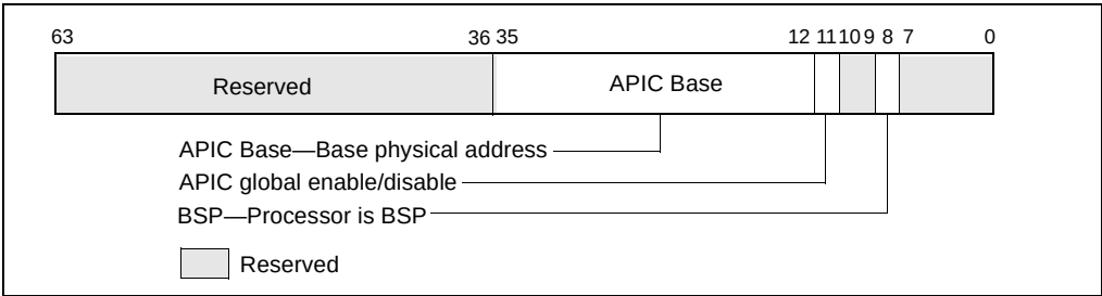
Figure 7-5. IA32_APIC_BASE MSR
