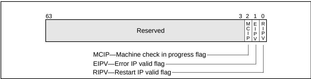
Figure 13-4. IA32_MCG_STATUS Register
