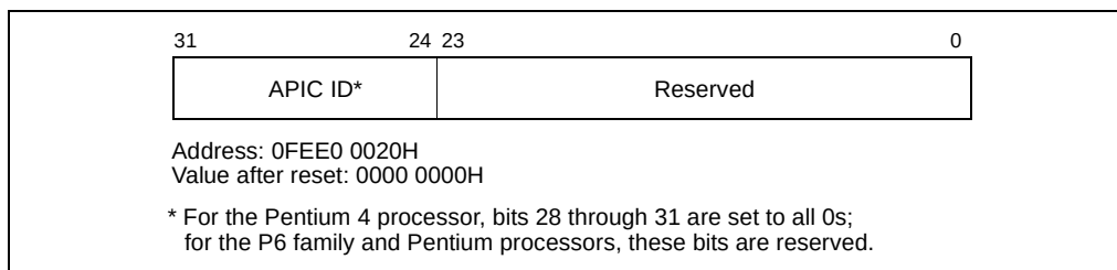
Figure 7-6. Local APIC ID Register
