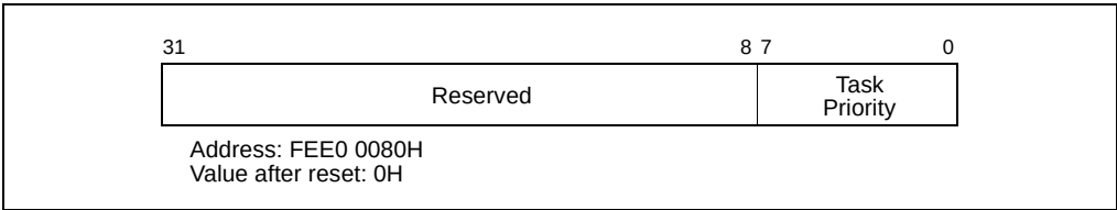
Figure 7-13. Task Priority Register (TPR)
