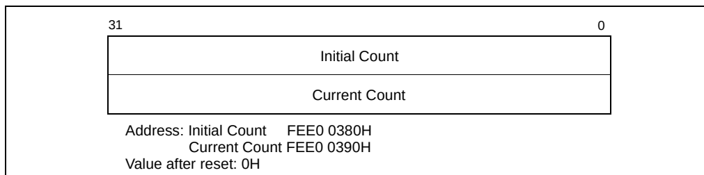
Figure 7-19. Initial Count and Current Count Registers
