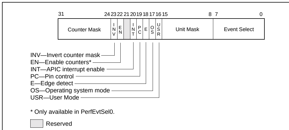
Figure 14-15. PerfEvtSel0 and PerfEvtSel1 MSRs
