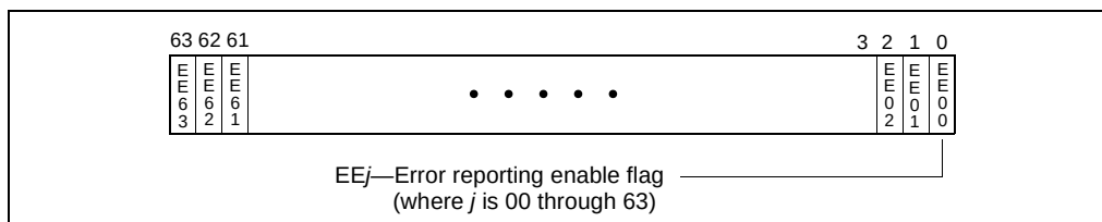
Figure 13-5. IA32_MCi_CTL Register
