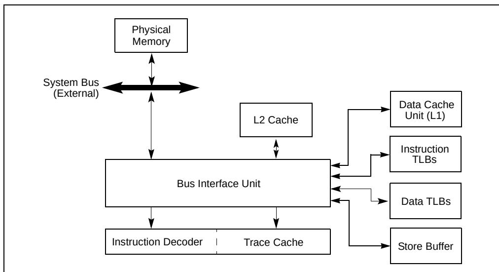
Figure 9-1. Pentium 4 Cache Structure
