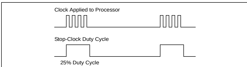
Figure 12-6. Processor Modulation Through Stop-Clock Mechanism
