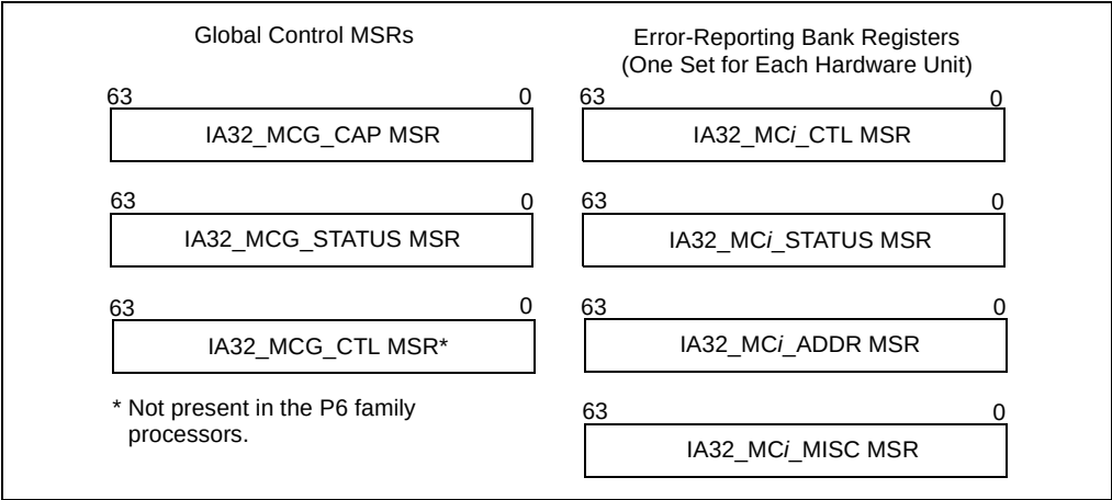
Figure 13-1. Machine-Check MSRs
