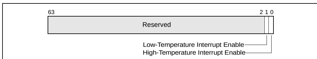
Figure 12-8. IA32_THERM_INTERRUPT MSR
