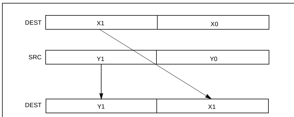
Figure 3-18. UNPCKHPD Instruction High Unpack and Interleave Operation
