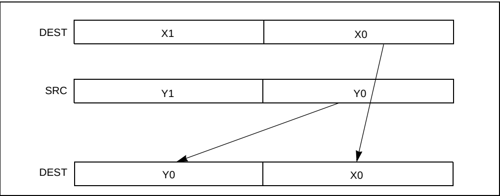
Figure 3-20. UNPCKLPD Instruction Low Unpack and Interleave Operation
