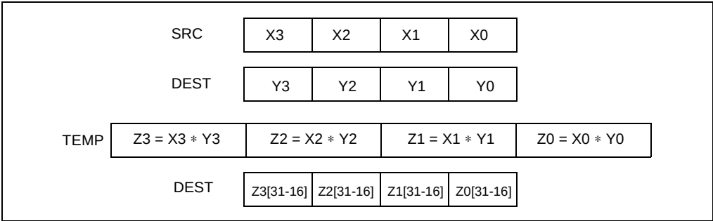
Figure 3-7. PMULHUW and PMULHW Instruction Operation Using 64-bit Operands
